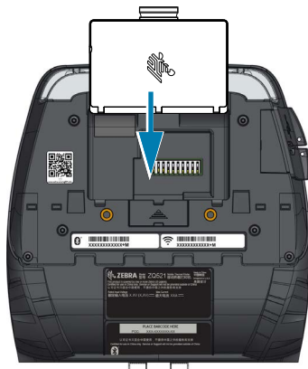
Figure 9 Battery Insertion
