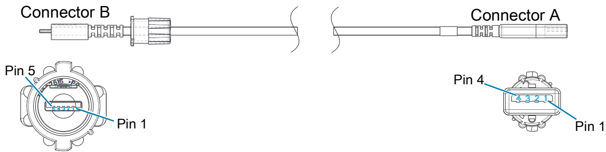
Figure 46 Micro,USB-A to USB-A
