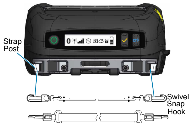
Figure 35 Hand Strap
