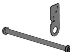
Rewinder Shaft Holder Bracket & Rewinder Bracket Shaft
