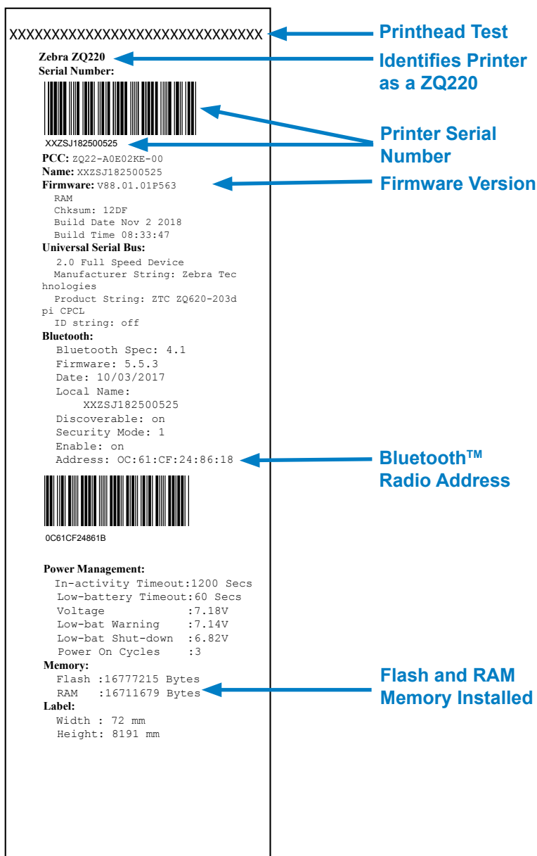
Figure 21 • Configuration Label
