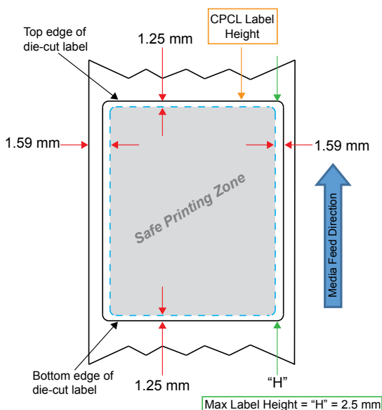
Figure 9 • Gap Media
