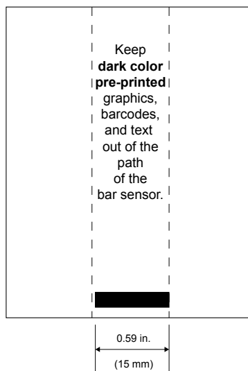
Figure 12 • Label Areas
