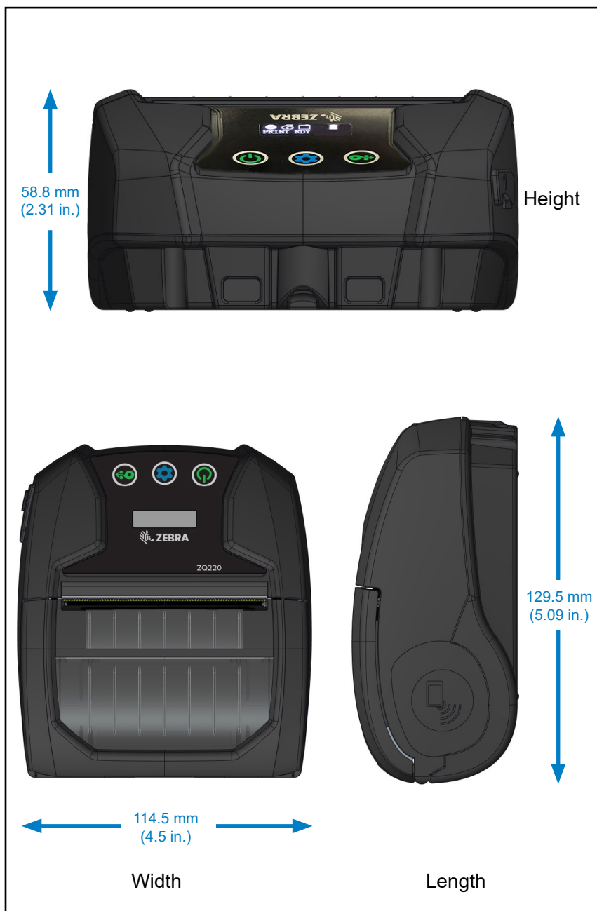
Figure 22 • Printer Dimensions
